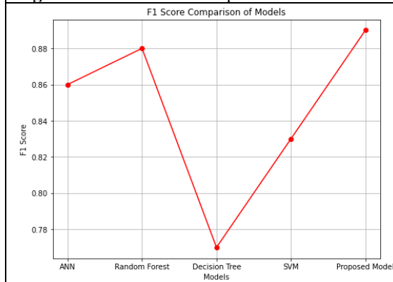
Figure 6. Performance comparison of models
